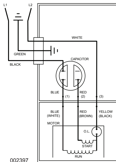
WIRING DIAGRAM FOR MODELS "N282-A", "N282-B" and "N282-C" "E282-A", "E282-B" and "E282-C" 11/81 (XM) to Current
